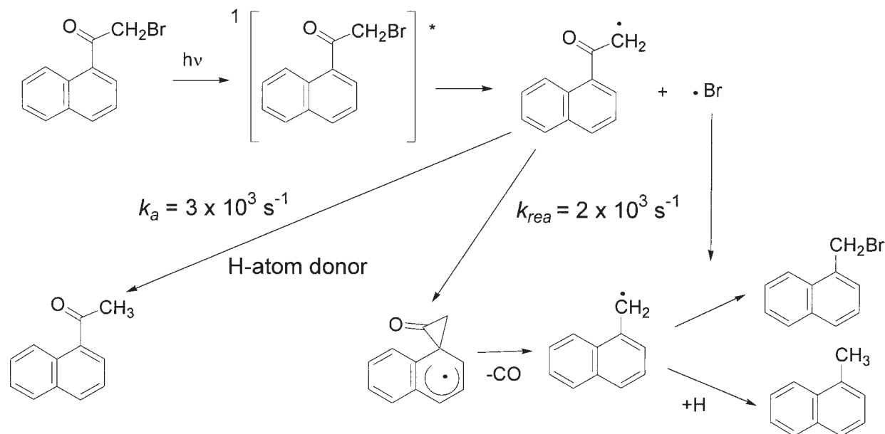
Fig. 8. Reaction scheme of a photochemical reaction of 1-BAN.
