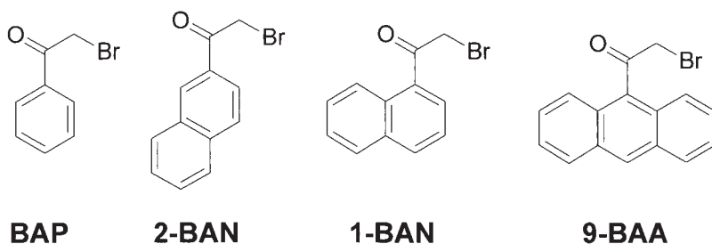
Scheme 2. Structures of \alpha -bromoacetylarenes investigated in this study.
