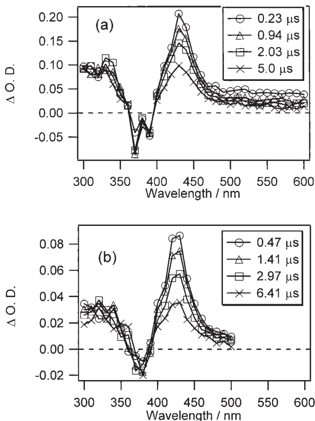
Fig. 7. Transient absorption spectra of 9-BAA in benzene (a) and in acetonitrile (b) under argon.
