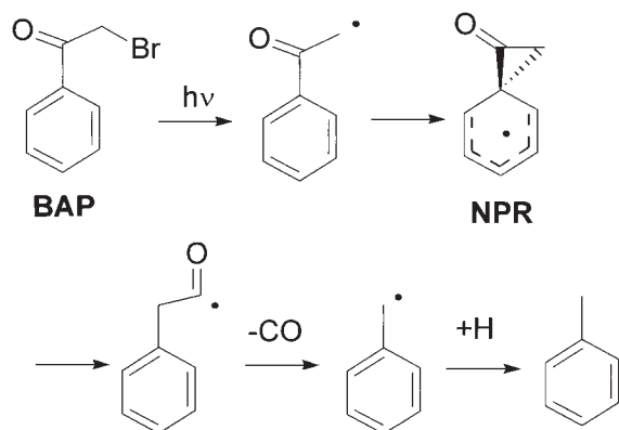
Scheme 1. Scheme of rearrangement reaction for BAP .
