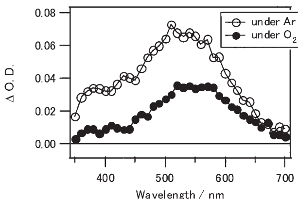
Fig. 3. Transient absorption spectra of 1-BAN in benzene at 400 ns after laser excitation.
