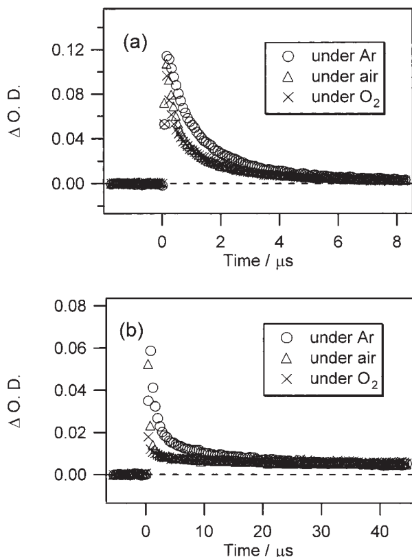
Fig. 4. Decay profiles of transient absorption monitored at 540 nm (a) and 400 nm (b) after the laser photolysis of 1-BAN in benzene.
