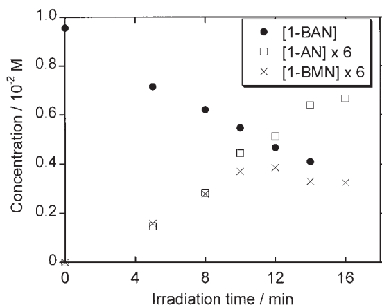
Fig. 1. Time profile of the ratio of the compounds determined by GC in photoreaction of 1-BAN in benzene.
