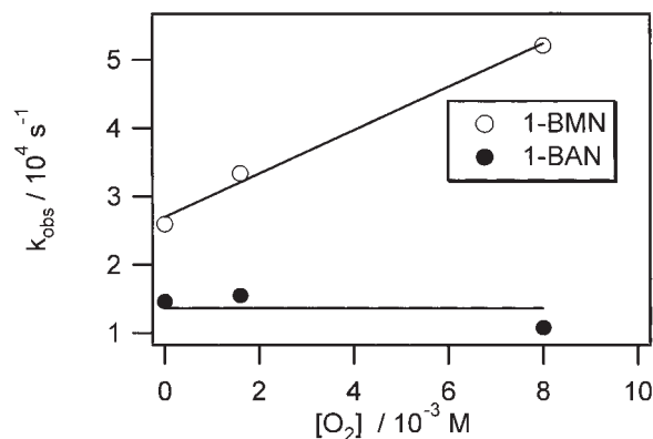
Fig. 5. Stern-Volmer plot of the radical quenching experiment observed by photolysis of 1-BAN and 1-BMN by oxygen in acetonitrile.
