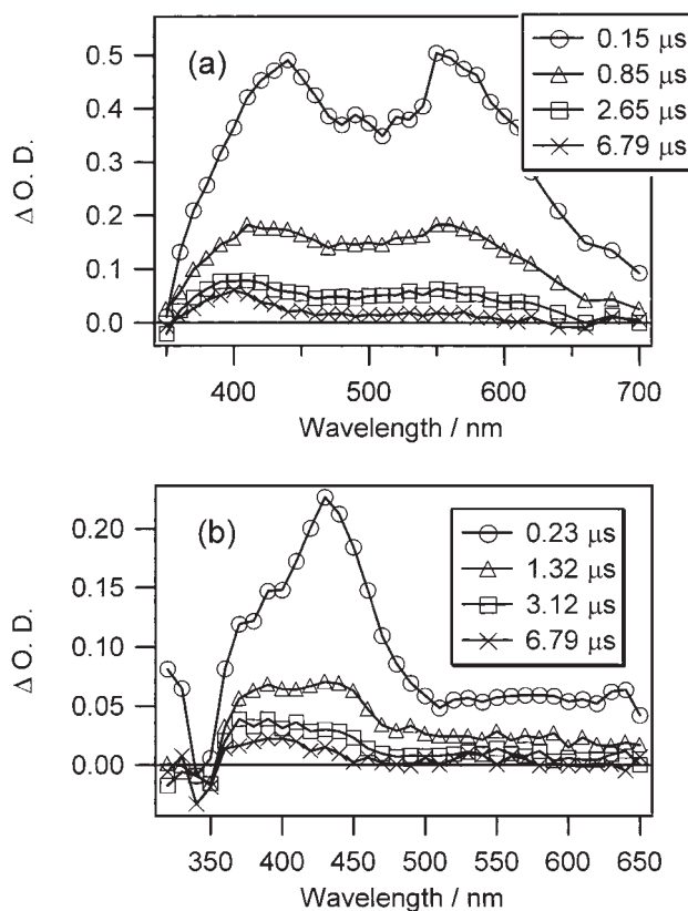
Fig. 6. Transient absorption spectra of 2-BAN in benzene (a) and in acetonitrile (b) under argon.
