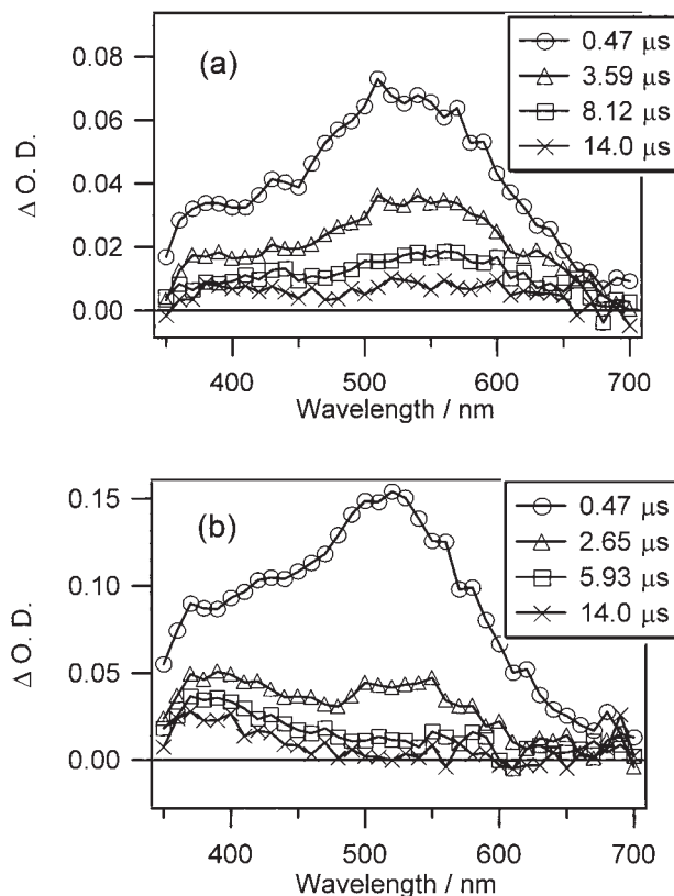
Fig. 2. Transient absorption spectra of 1-BAN in benzene (a) and in acetonitrile (b) under argon.
